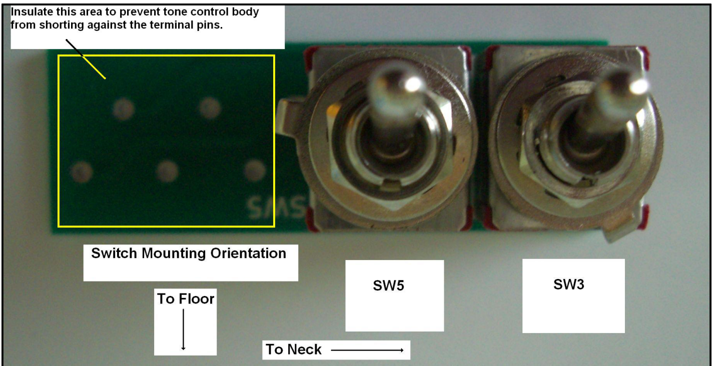
Figure 5 – T2P-Switch Orientation
