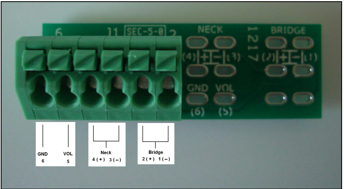
Figure 4 – T2P-Switch Green Terminal Strip Designation
